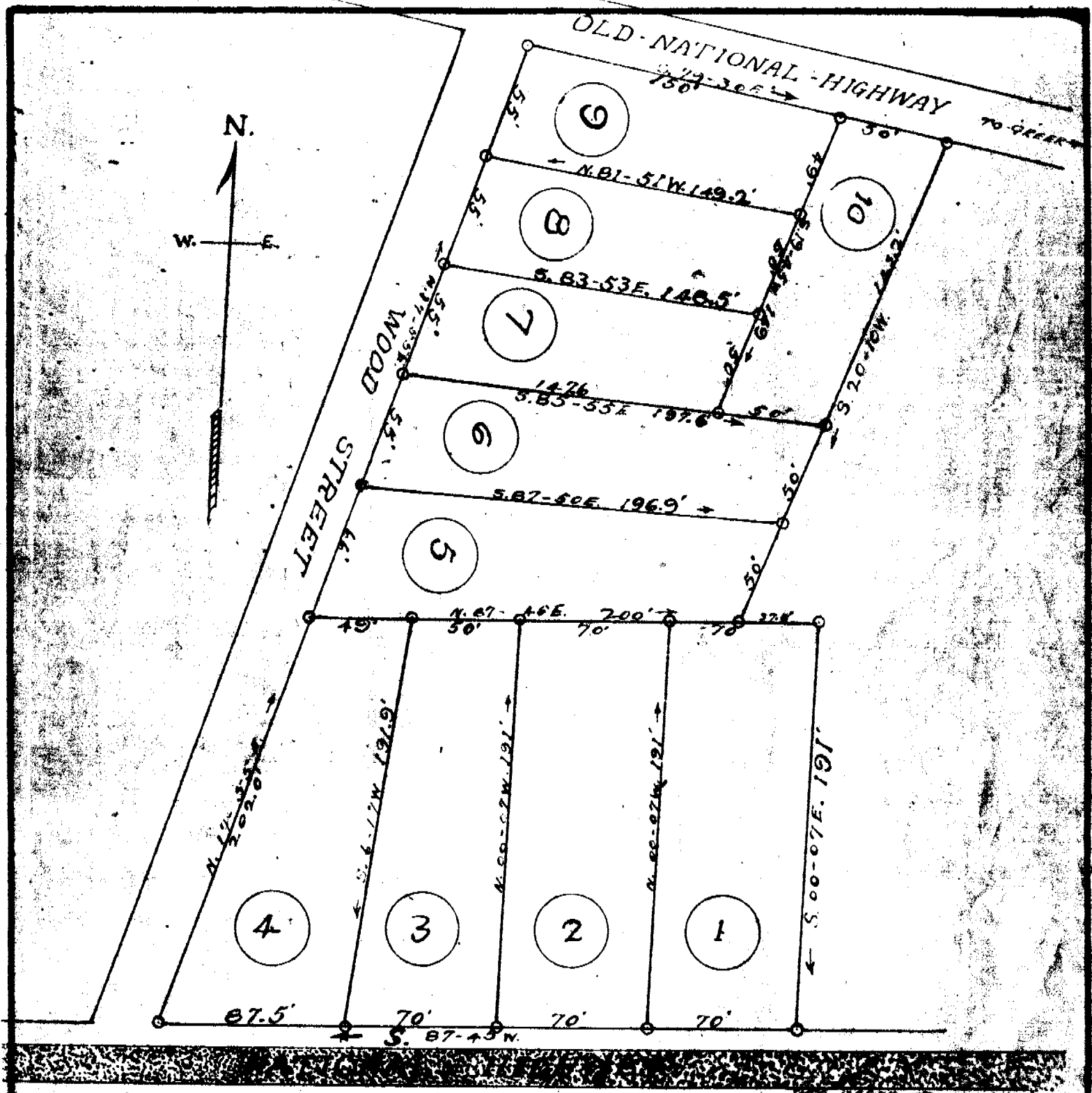
MAP OF H. J. LANFORD PROPERTY NEAR GREER S. C. SURVEYED AND PLATTED BY H. S. BROCKMAN, SURVEYOR MARCH 27 1928 SCALE: 1" = 50 FT
